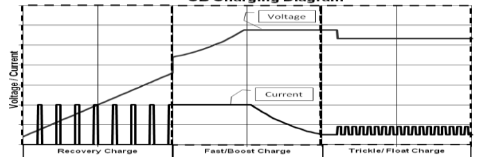
CB Charging Diagram
